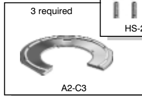
Membrane clamp ring with integral gravel stop and combination underdeck clamp and extension. HS-2 hardware set included.
