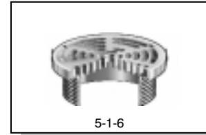
5" (125) diameter, 1/4" (6) thick, standard reinforced nickel bronze strainer with vandal proof screws
